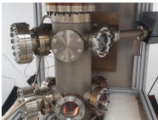
UHV Bakeout Facility
